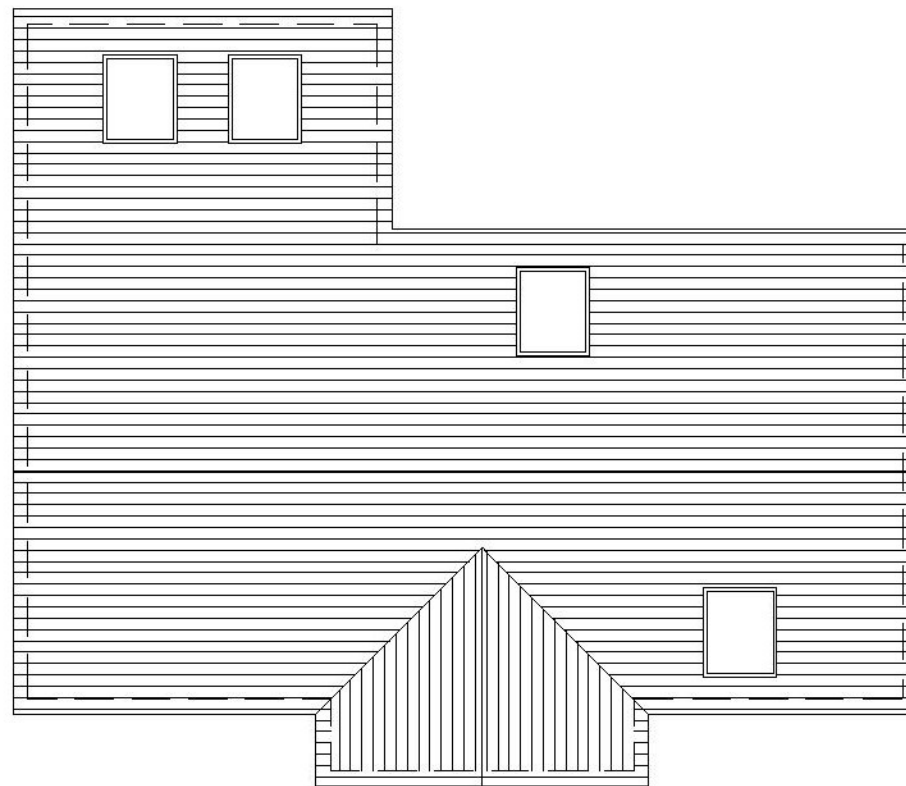
ROOF PLAN
